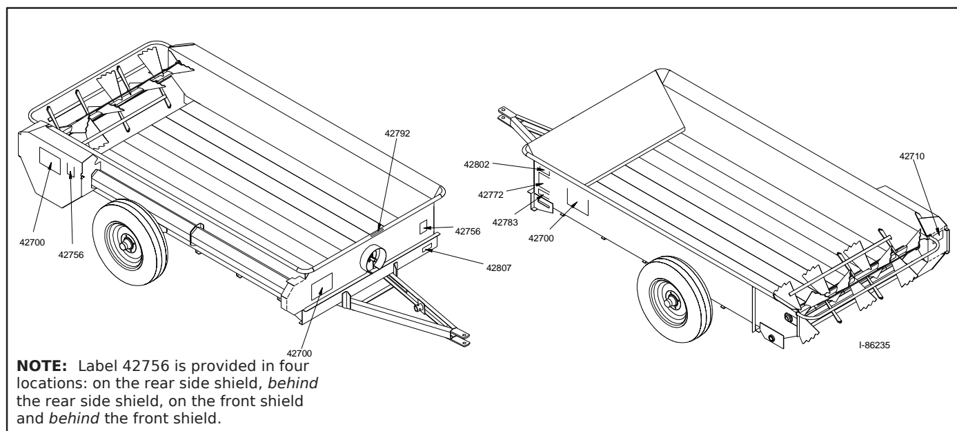
Figure 1A - Spreader Safety Label Locations
